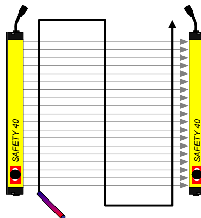
Figure 2: Check of the protective field using a test bar
